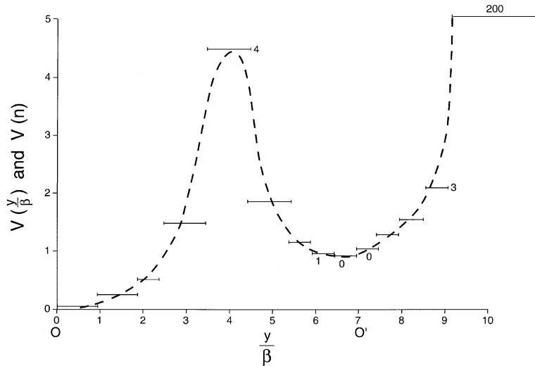
Fig. 4. The broken line represents the function V , Eq. (20), which is a measure of the complex phase velocity V_c , Eq. (24), describing an avalanching granular bed. The depth of the channel h_s corresponds to the point O' . The horizontal bars depict the intervals in which the linearized wave Eq. (4) can be assumed to hold. V_n is the phase velocity at the center of the n th interval. To the left of O , V = 333 m/s, i.e., the phase velocity in air at standard conditions.
