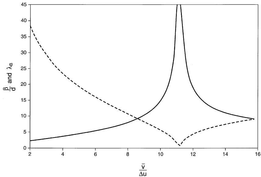
Fig. 11. Plots of \beta/d , Eq. (12), solid line and of \lambda_B = d/s , Eq. (27), broken line, versus the velocity ratio \bar{v}/\Delta u for: \mu = 0.5 , e = 0.85 , \Delta = 0.6 and V_s = 1 m/s. For \bar{v}/\Delta u > \bar{v}/\Delta u|_o = 11.2 , where \beta/d \rightarrow \infty , the value of \beta/d shown has to be multiplied by \sqrt{-1} . Further, the part of the plot with \lambda_B < 5 , about, is not applicable since Eqs. (A.16a)–(A.16c) are not applicable when s \rightarrow d .
