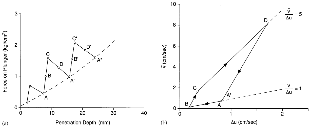
Fig. 14. (a) Rough sketch of the force experienced by the plunger versus penetration depth in a bed of sonorous sand for an experimental arrangement similar to that shown in Fig. 3, based on Fig. 9 in Miwa et al. (1983). The broken line corresponds to a silent sand. (b) A hypothetical hysteresis loop of \bar{v} versus \Delta u , corresponding to the plot in part (a). The lengths of the various intervals are not necessarily analogous to the lengths of the corresponding time intervals. The slopes \bar{v}/\Delta u = 5 and 1 correspond to the singing and silent sands, respectively. The intervals AB and CD correspond to the stages of compactness and delatancy, respectively. The acoustic emission occurs during the latter part of the interval CD .
