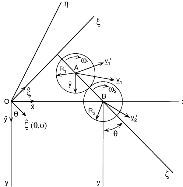
Fig. 15. Schematic of the collision of two spheres, A, B , of radii R_1, R_2 , respectively. The velocities after collision are indicated with a prime. The laboratory frame is shown by the axes xyz , with \hat{z} out of the plane of the paper. The \zeta axis is along the surface-normal at the point of contact. \hat{\zeta} has polar and azimuthal angles \theta, \phi in the xyz axes. \hat{\eta} = \hat{\xi} \times \hat{\zeta} .
