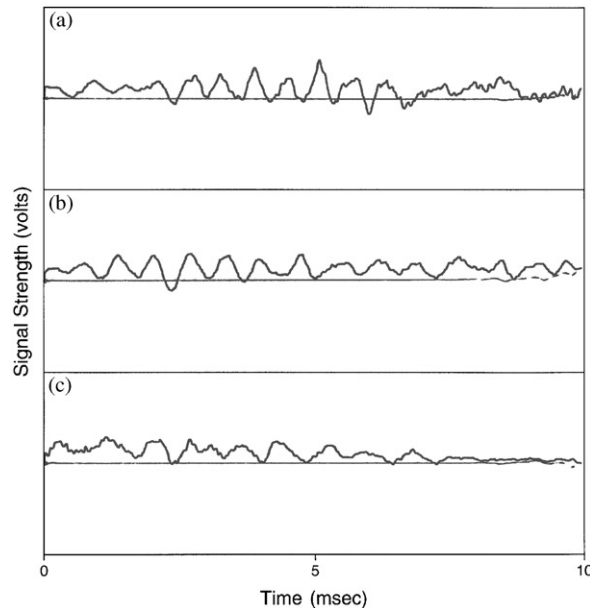
Fig. 13. (a) Time signal after several light impactions at the same point on an approximately 2 cm deep by 20 cm in diameter pile of nearly silent sand from Lake Michigan placed on a hard surface. The final depression had depth of about 0.7 cm at the center and diameter of about 5 cm at the top. (b) Same as part (a) with an otherwise silent beach sand, d \approx 0.4 mm. (c) Same as part (a) with a coarser, nearly silent sand placed on a 2.5 cm thick foam pad.
